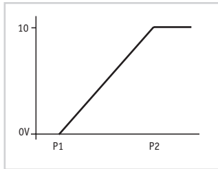
Uscita analogica in tensione/Power voltage analogical output
