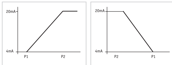
Uscita analogica in corrente/Current analogical output
