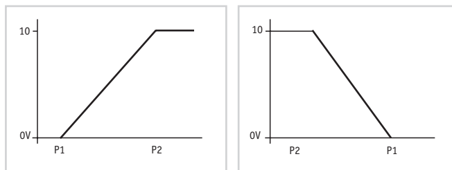
Uscita analogica in tensione/Power voltage analogical output
